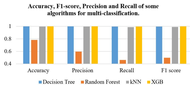
Figure 4. Accuracy, F1-score, Precision and Recall of some algorithms for multi-classification
