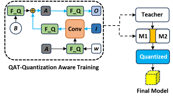
Figure 1. Quantization Applied to both Teacher and Student Model. F_Q = Fake Quantization, W = Weights, A = Activation Function, B = Bias, O = Output, I = Input
