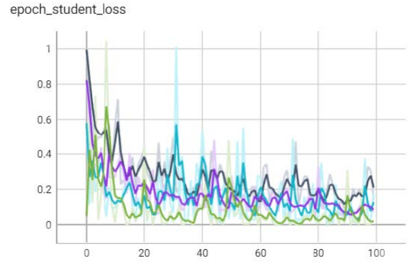
Figure 5. Student loss in multiple tuning stages.
