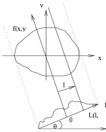
Figure 6. Geometric representation of lines and projections.
