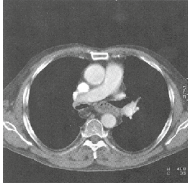
Figure 5. Visualization of the projection slice theorem.
