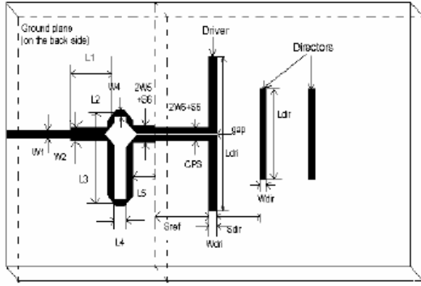
Fig.1- Schematic of the enhanced (2 directors) antenna
