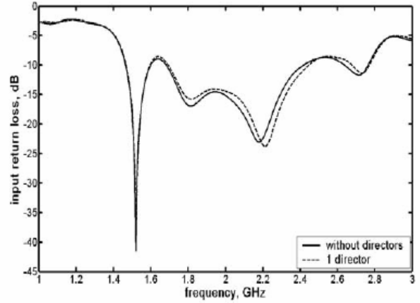
Fig.6. Comparing the antenna without director to the antenna with one director
