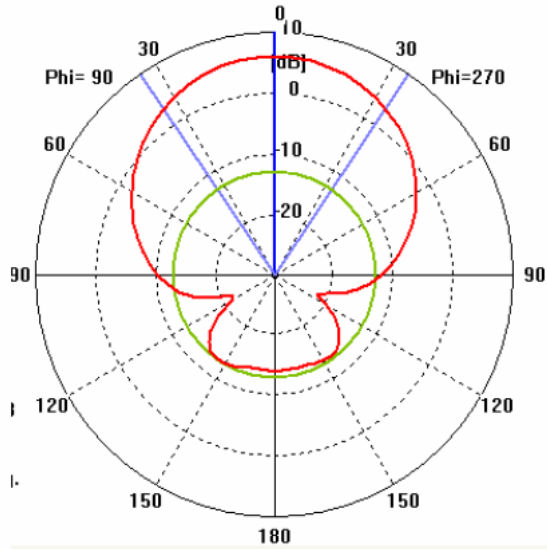
Fig.3. Antenna radiation pattern at 2.1GHz
