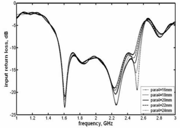
Fig.11. Simulation results of various values of parameter 4 - S_{dir}
