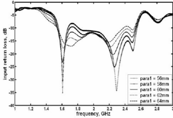
Fig.5. Simulation results of various values of parameter 1
