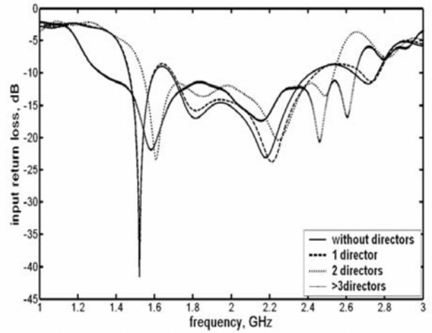
Fig.8. Simulation results of antenna models with different directors
