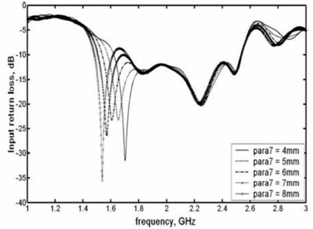
Fig.14. Simulation results of various values of parameter 7- L_4
