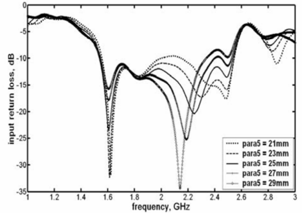
Fig.12. Simulation results of various values of parameter 5 - S_{ref}
