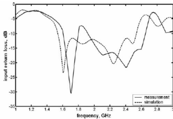
Fig.16. Input return loss of fabricated UMTS quasi-Yagi antenna
