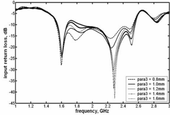
Fig. 10. Simulation results of various values of parameter 3 - S_6
