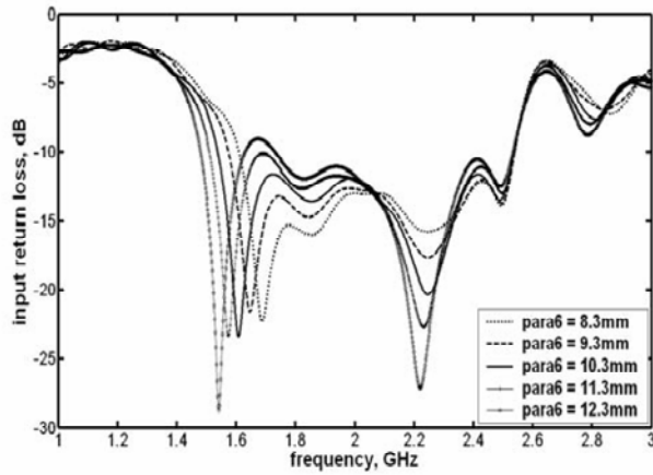
Fig.13. Simulation results of various values of parameter 6- L_5
