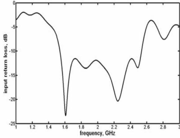
Fig. 2. Antenna input return loss
