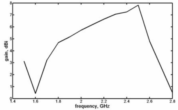
Fig.4. Gain of the designed antenna
