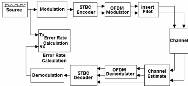
Figure. 1. STBC MIMO-OFDM system with pilot-aided method
