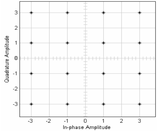
Figure 3. Received 16-ary QAM constellation without any impairment
