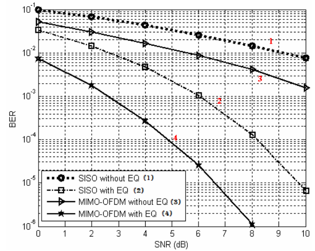
Figure 6. The plot of BER vs SNR of four scenarios
