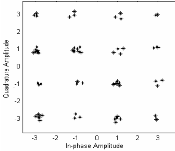
Figure 5. Received 16-ary QAM constellation with AWGN plus multipath fading after the Equalizer block
