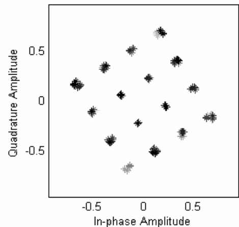
Figure 4. A snap shot of the received 16-QAM constellation with multipath fading
