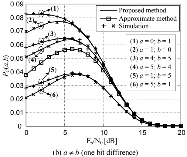
Fig. 4. Codeword transition probability P_C(a, b) evaluated by different methods (in the case of N=128 , M=16 )
