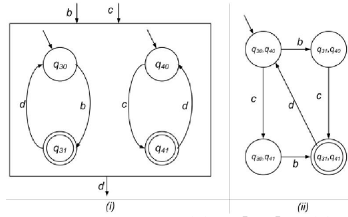
Figure 3: TCIA Q where J_Q(b) = [2, 3] , J_Q(c) = [1, 3] , J_Q(d) = [2, 4] (i) and it's state transition graph (ii) is compatible with TCIA P in Example 2
