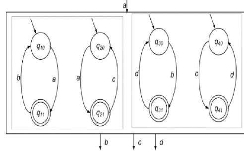
Figure 4: The result of parallel composition of P and Q in Figure 2 and 4
