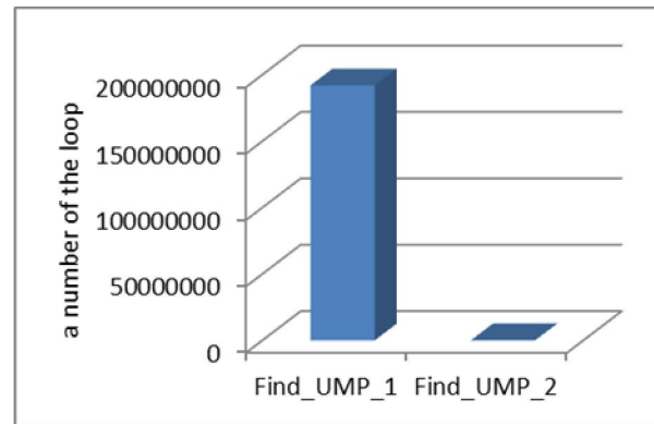
Figure 3: Compare the number of the loop of two algorithms
