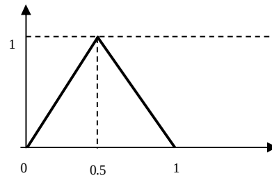
Fig. 1. Fuzzy number about_0.5
