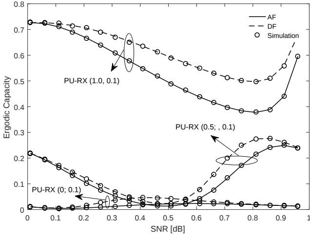
Figure 4. Effect of relay locations on the system ergodic capacity.
