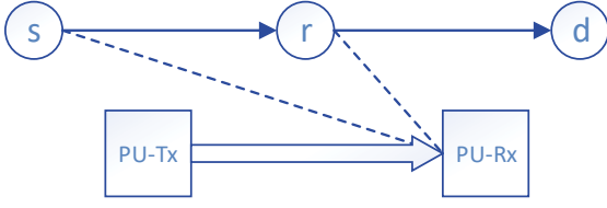
Figure 1. Cognitive underlay AF relay network.
