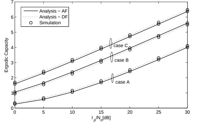
Figure 2. Ergodic capacity versus average SNRs.
