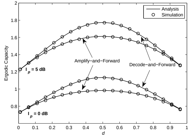
Figure 3. Effect of relay locations on the system ergodic capacity.
