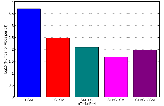
Figure 2. Complexity comparison between GC-SM, STBC-SM, STBC-CSM, SM-DC, and ESM at the spectral efficiency of 5 bpcu, SNR of 10 dB, with four transmit antennas, four receive antennas, and T = 60 symbol periods.
